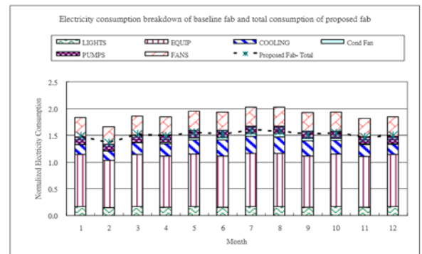
Figure 3. Energy simulation for building and industrial process
