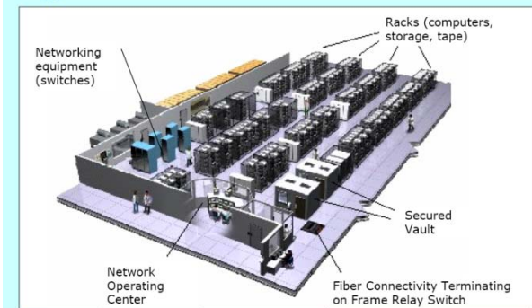
A Typical Data Center Raised Floor
