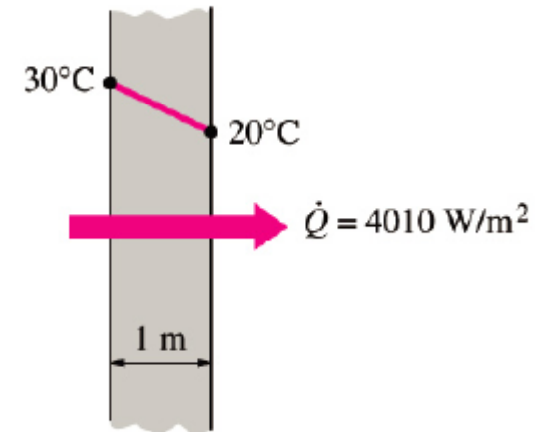
(a) Copper ( k = 401 \text{ W/m}\cdot^\circ\text{C} )
