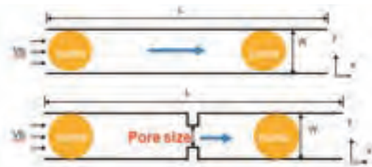
微流道兩相流 Microchannel two-phase flow
