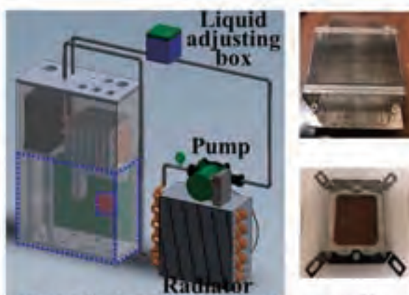
浸沒式冷卻 Immersion cooling
