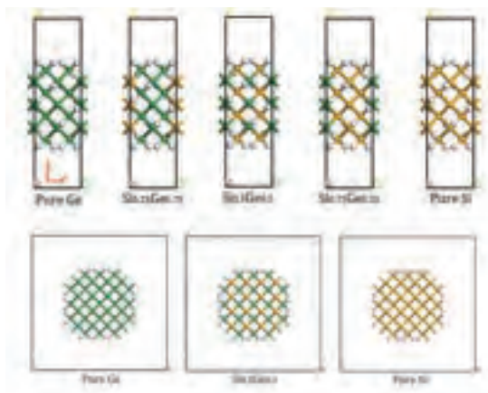
矽鍺超晶格奈米線電子傳輸 Si-Ge superlattice nanowire electron conductivity
