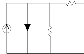
Solar cell DC circuit equivalent
