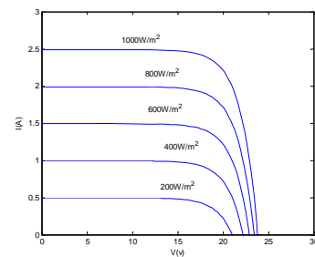
Solar cell V-I curve
